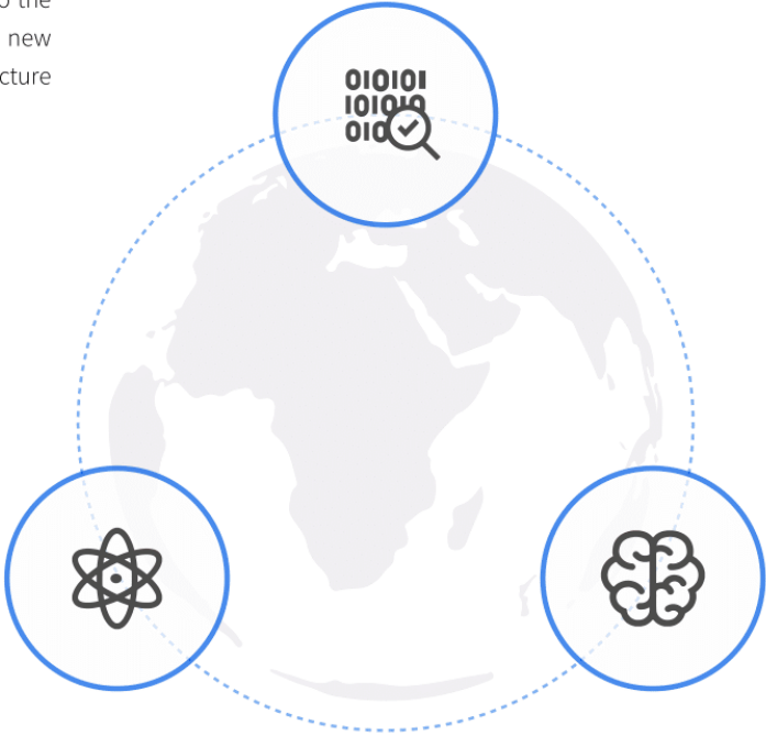
Machine learning
